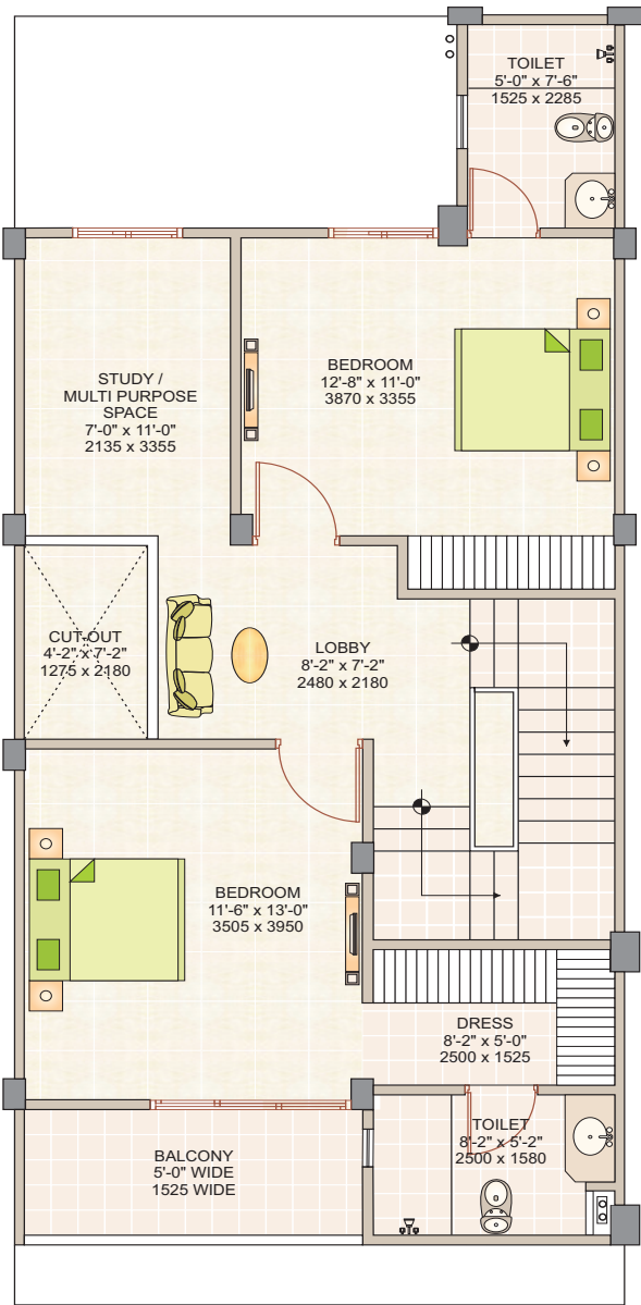
FIRST FLOOR
