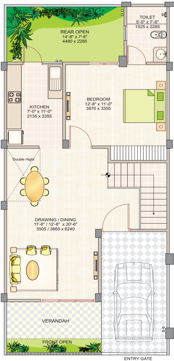
GROUND FLOOR
